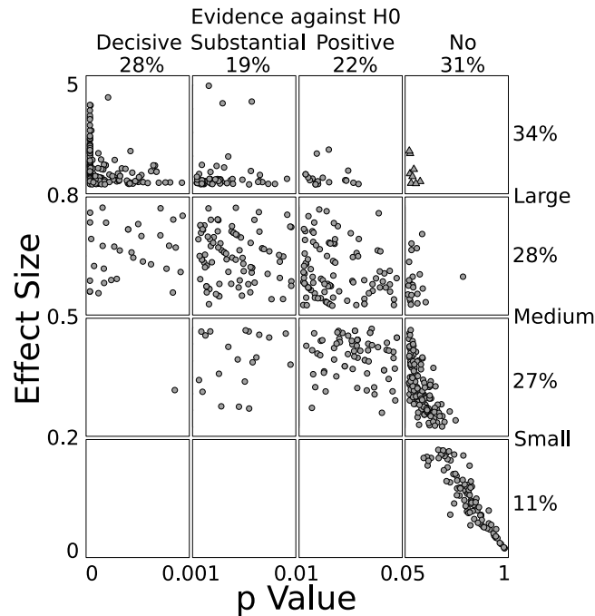
Figure 1. The relationship between effect size and p values. Points denote comparisons (855 in total). Points denoted by circle indicate relative consistency between the effect size and p value, while those denoted by triangles indicate gross inconsistency. The scale of the axes is based on the decision categories, as given in Table 1 and Table 2.
