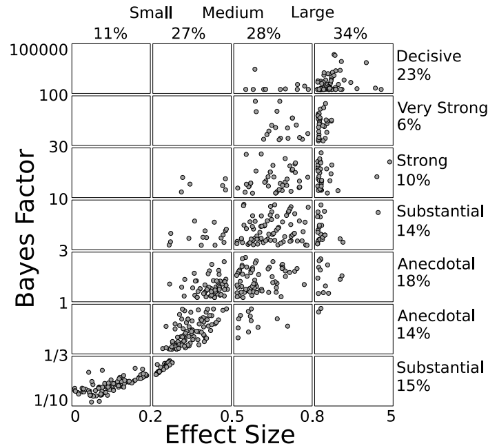
Figure 2. The relationship between Bayes factor and effect size. Points denote comparisons (855 in total). The scale of the axes is based on the decision categories, as given in Table 2 and Table 3.
