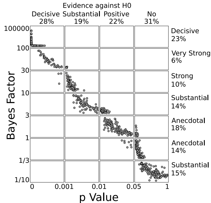
Figure 3. The relationship between Bayes factor and p value. Points denote comparisons (855 in total). The scale of the axes is based on the decision categories, as given in Table 1 and Table 3.
